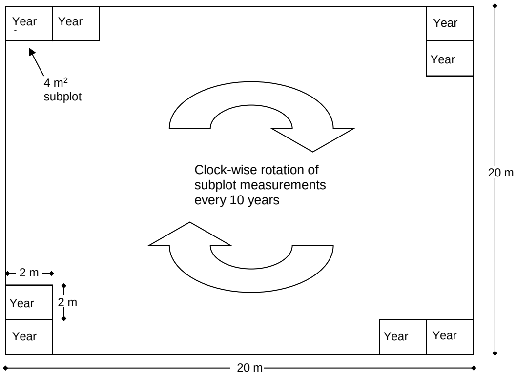
Figure 5. Example of a 400 m 2 sampling plot, also showing the 4 m 2 subplots therein (4 per measurement period every 10 years).
